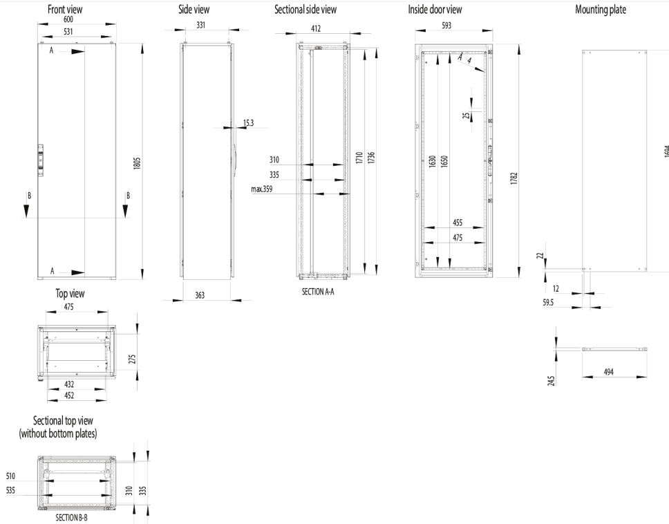
Dimension Diagram
