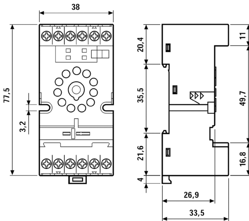
Dimension Diagram
